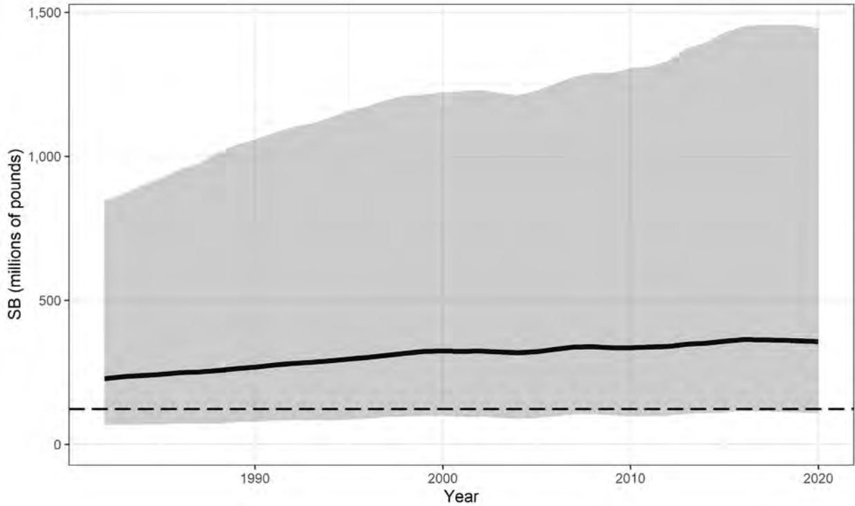
Figure 107. Spawning biomass estimated in JABBA-Select. The solid line is the median and the shaded region is the 95% credible interval. The dashed line is the median SB_{MSY} estimate. Note: Figure has been updated in Section 13.5 based on changes that were made to the base model configuration in response to the recommendations of the Peer Review Panel.
