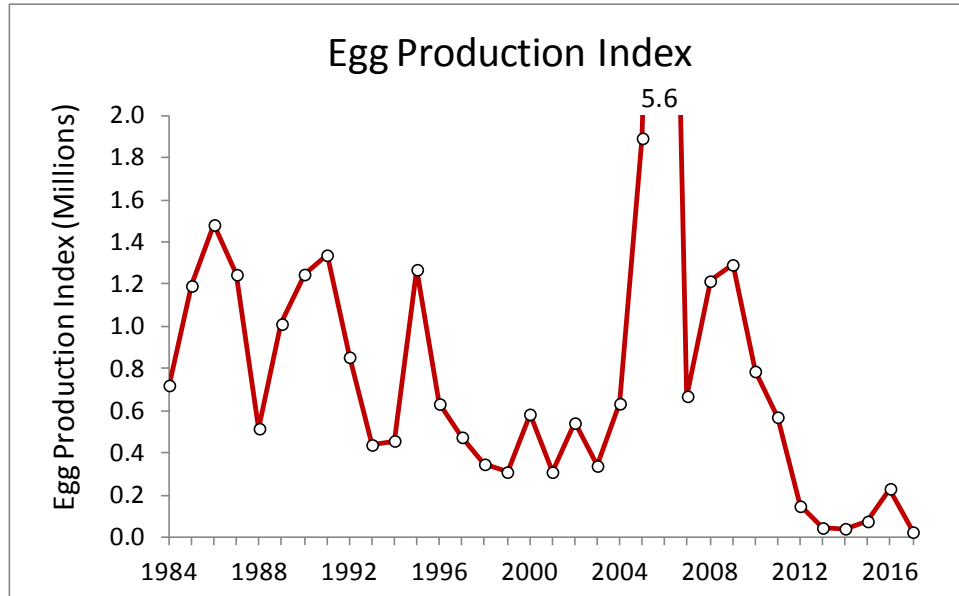
Figure 16: Egg production index for Gulf of Maine northern shrimp based on stratified mean number of females at length from the summer shrimp survey and estimated fecundity at length (Haynes and Wigley 1969). Index for 2006 (off scale) was 5.6 million.
