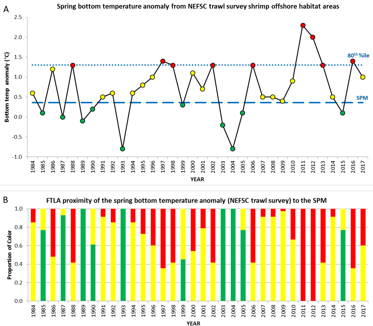
Figure 29: Traffic light analysis of spring bottom temperature anomalies from the NEFSC trawl survey. (A) Spring bottom temperature anomaly (°C) from the NEFSC trawl survey in shrimp offshore habitat areas from 1984–2017, with ‘stable period’ (1985–1994) mean (SPM) (dashed) and 80th percentile of the time series from 1984–2017 (dotted) indicated. Green values \leq SPM; red values \geq 80th percentile; yellow values > SPM and < 80th percentile. (B) Fuzzy Traffic Light Analysis (FTLA) color proportions indicate proximity of annual indices to the SPM (red = unfavorable; green = favorable).
