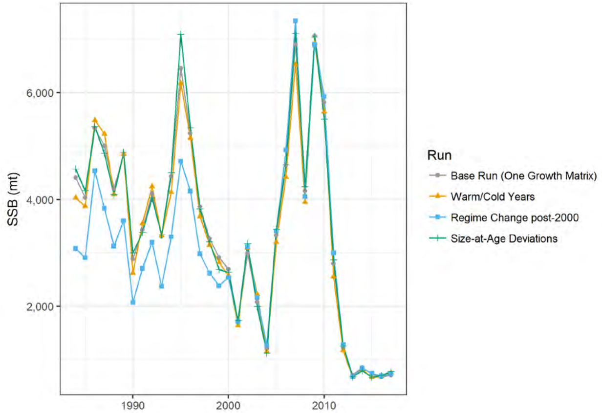
Figure 5.50. Estimates of SSB from the UME model under different growth block scenarios.
