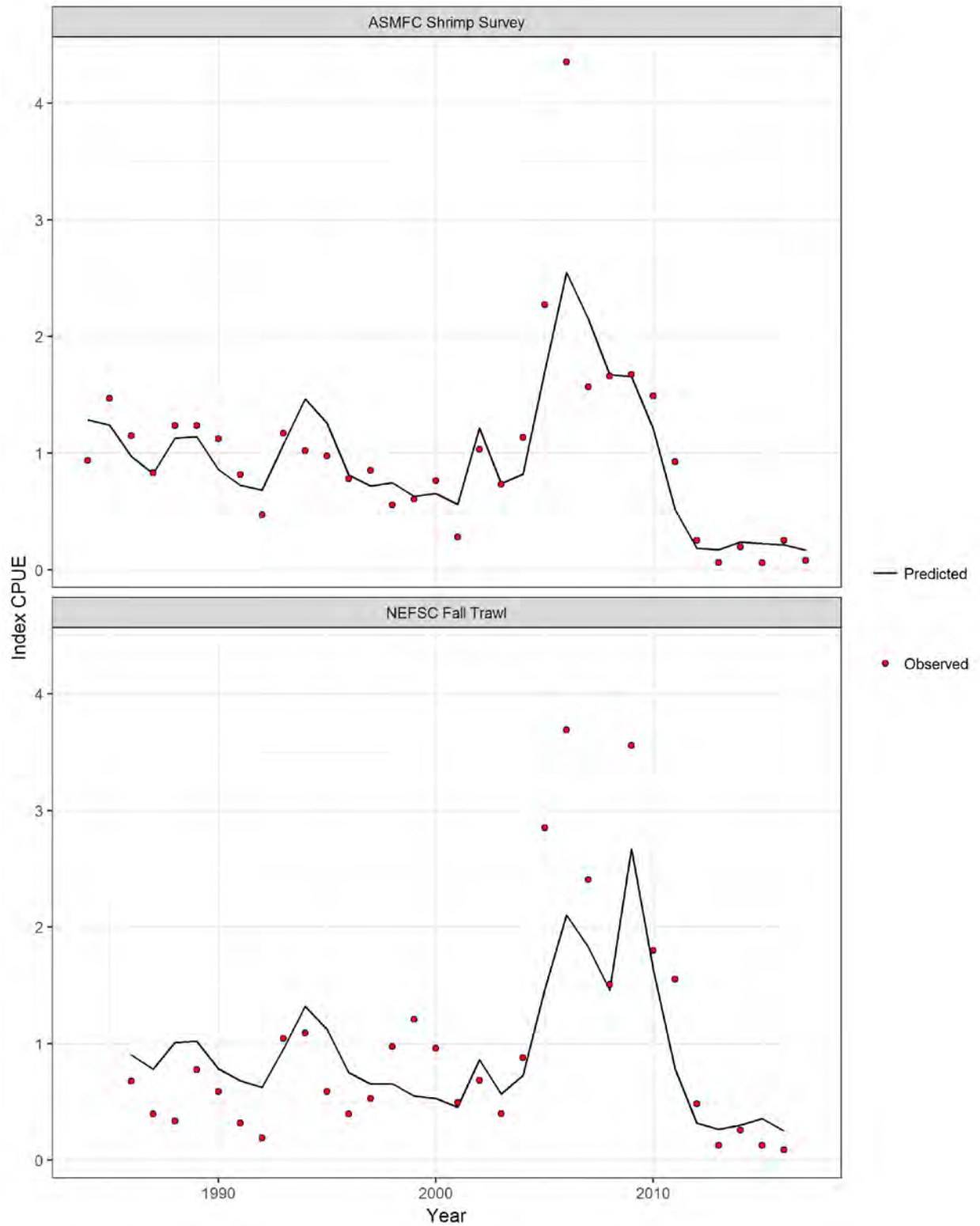
Figure A10. Observed and predicted index values for the ASMFC shrimp survey (top) and the NEFSC Fall Trawl Survey (bottom).
