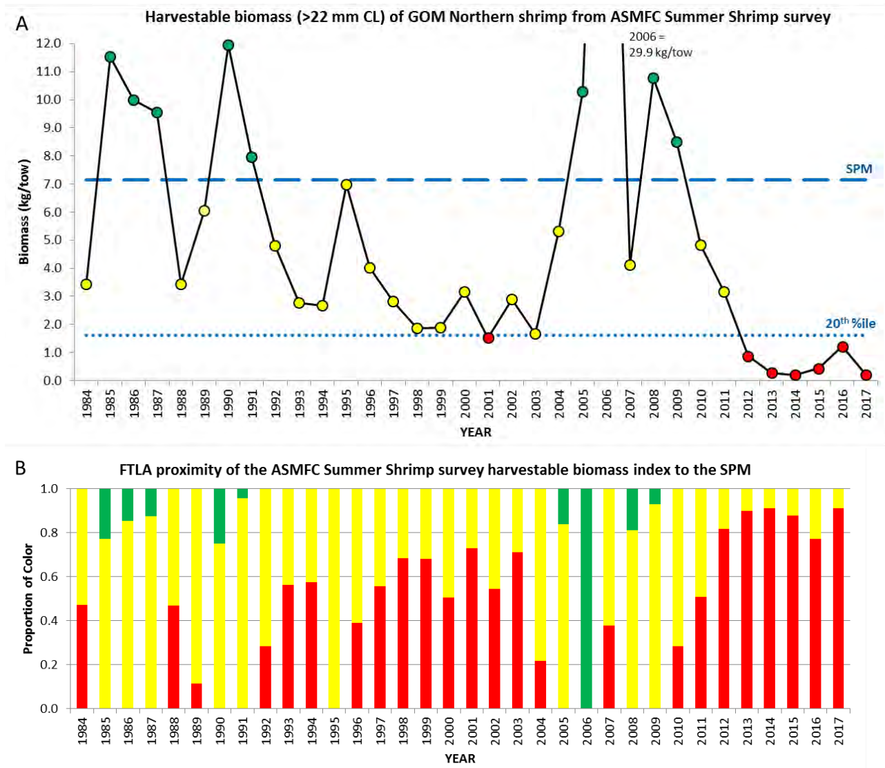
Figure 5.66 Traffic light analysis for harvestable biomass. (A) Harvestable biomass of Gulf of Maine northern shrimp from the ASMFC Summer Shrimp survey 1984–2017, with ‘stable period’ (1985–1994) mean (SPM) (dashed) and 20th percentile of the time series from 1984–2017 (dotted) indicated. Green values \geq SPM; red values \leq 20th percentile; yellow values > 20th percentile and < SPM. (B) Fuzzy Traffic Light Analysis (FTLA) color proportions indicate proximity of annual indices to the SPM (red = unfavorable; green = favorable).
