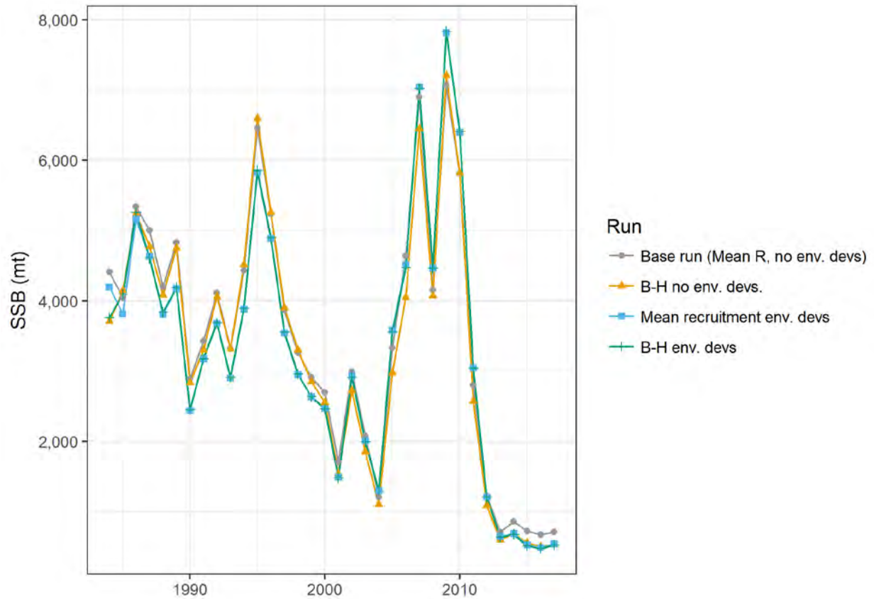
Figure 5.39. SSB estimates from the UME model fit with and without an environmental index of recruitment deviations.
