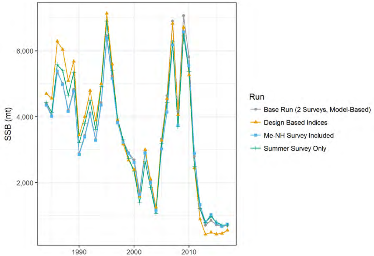
Figure 5.44. Estimates of SSB from the UME model under different index scenarios.
