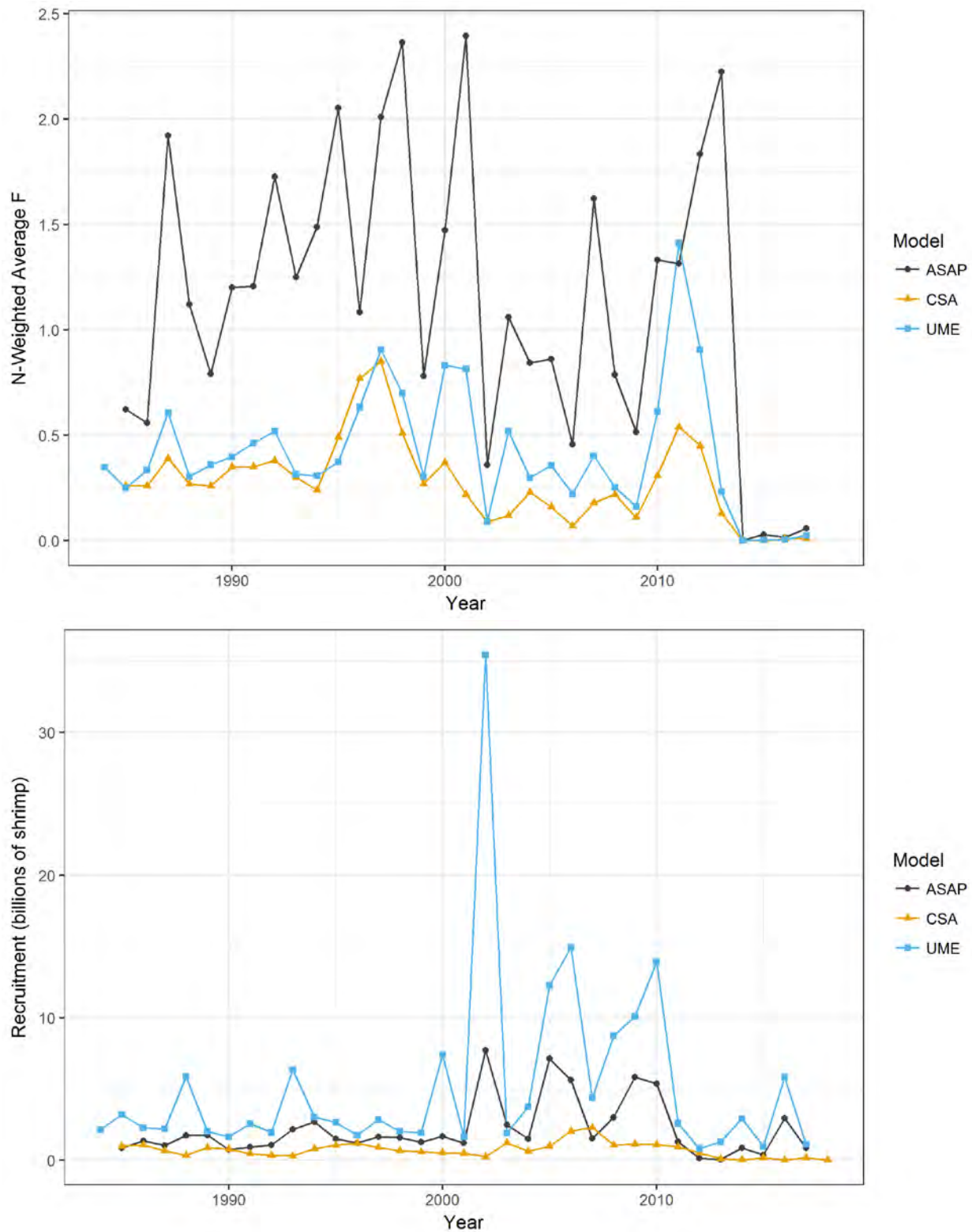
Figure A25. Comparison of fishing mortality (top) and recruitment estimates (bottom) from the new base run, the new ASAP run, and the original CSA run.
