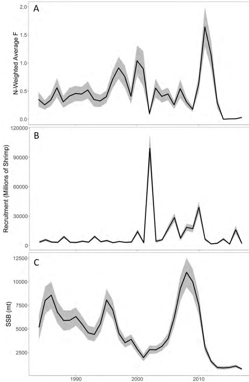
Figure 7. Estimates of A) fishing mortality rates, B) recruitment and C) spawning stock biomass of Northern Shrimp from the base run of the UME model. Grey shading indicates 95% confidence intervals of the estimates. (From 2018 Northern Shrimp Benchmark Assessment)
