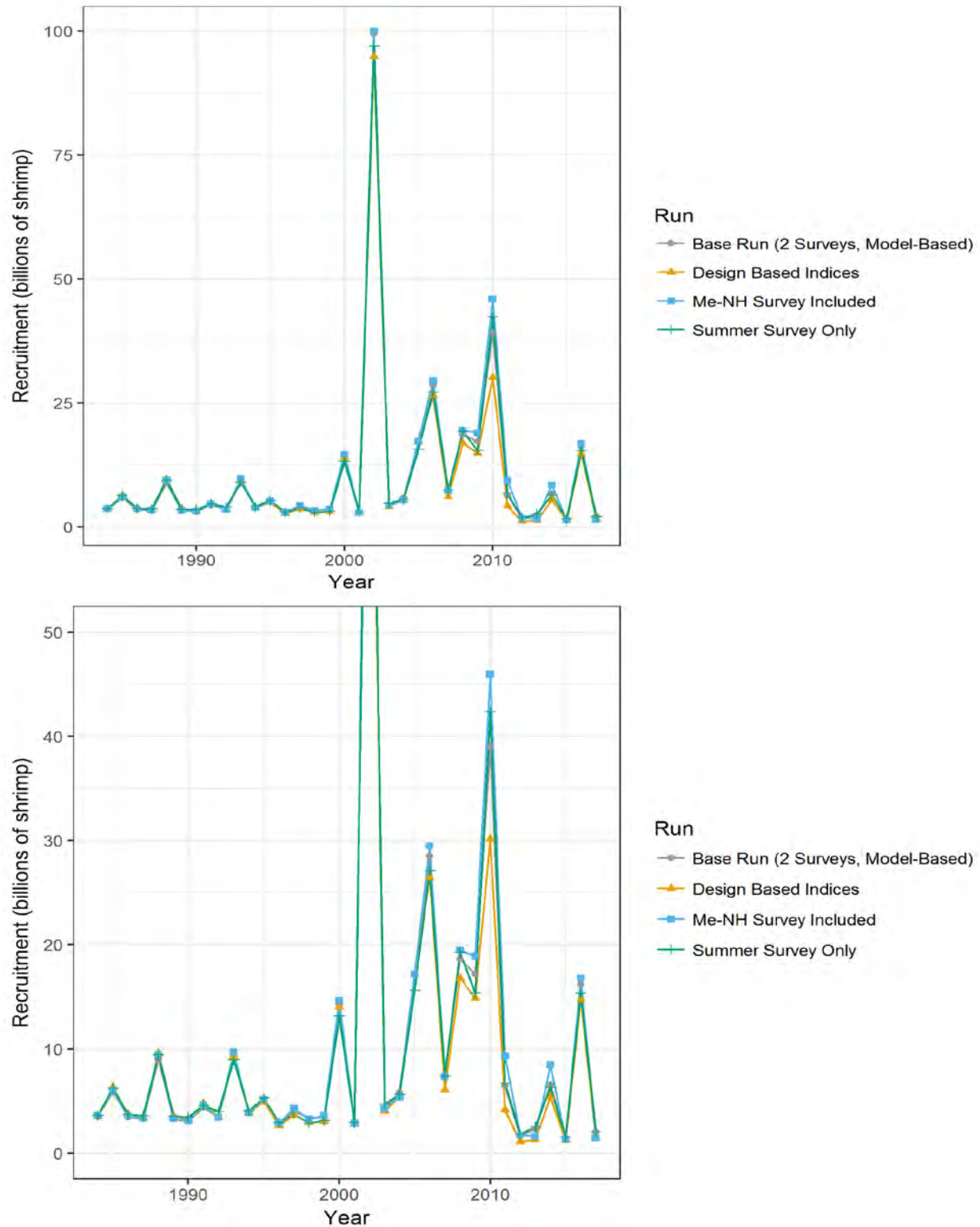
Figure 5.45. Estimates of recruitment from the UME model under different index scenarios. The y-axis on the second graph has been truncated to show detail.
