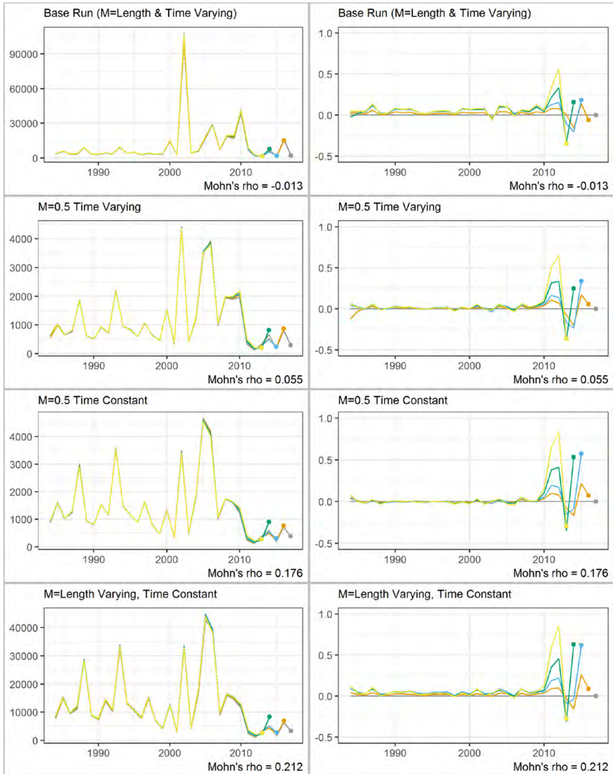
Figure 5.33. Retrospective patterns in recruitment from the UME model under different M scenarios.
