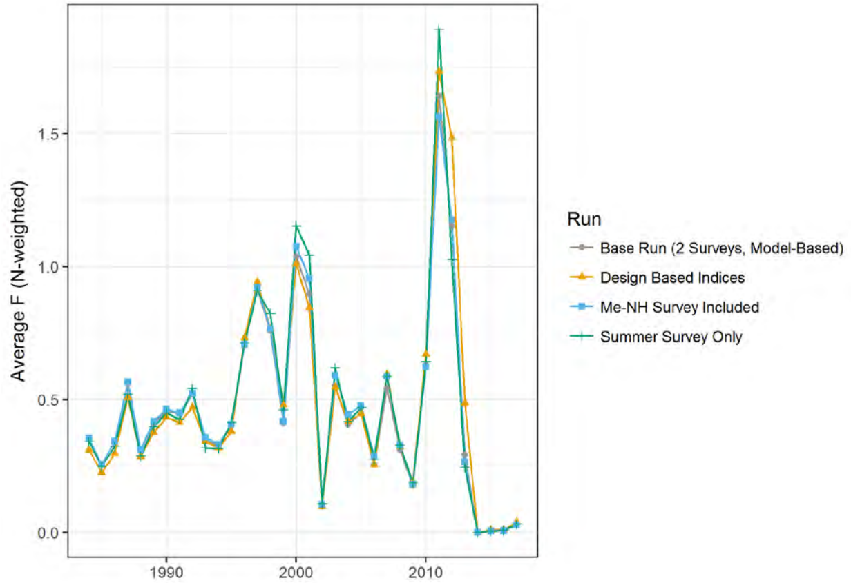
Figure 5.46. Estimates of average F from the UME model under different index scenarios.
