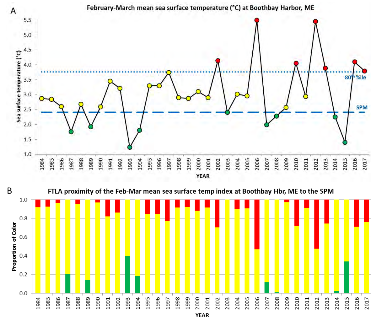
Figure 5.74 Traffic light analysis of Feb-Mar sea surface temperature at Boothbay Harbor, ME. (A) February to March mean sea surface temperature (°C) at Boothbay Harbor, ME from 1984–2017, with ‘stable period’ (1985–1994) mean (SPM) (dashed) and 80th percentile of the time series from 1984–2017 (dotted) indicated. Green values \leq SPM; red values \geq 80th percentile; yellow values > SPM and < 80th percentile. (B) Fuzzy Traffic Light Analysis (FTLA) color proportions indicate proximity of annual indices to the SPM (red = unfavorable; green = favorable).
