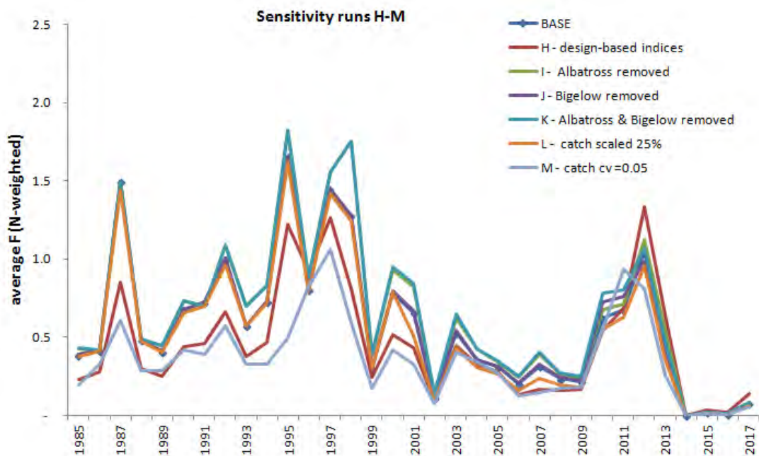
Figure 5.65 (a-b). ASAP model generated estimates of average F for base and sensitivity runs. a) base model compared to alternative natural mortality scenarios; b) base model compared to runs with changes in survey indices, catch, and catch CVs; See Table 4.1 for descriptions of sensitivity runs (i.e. scenarios).
