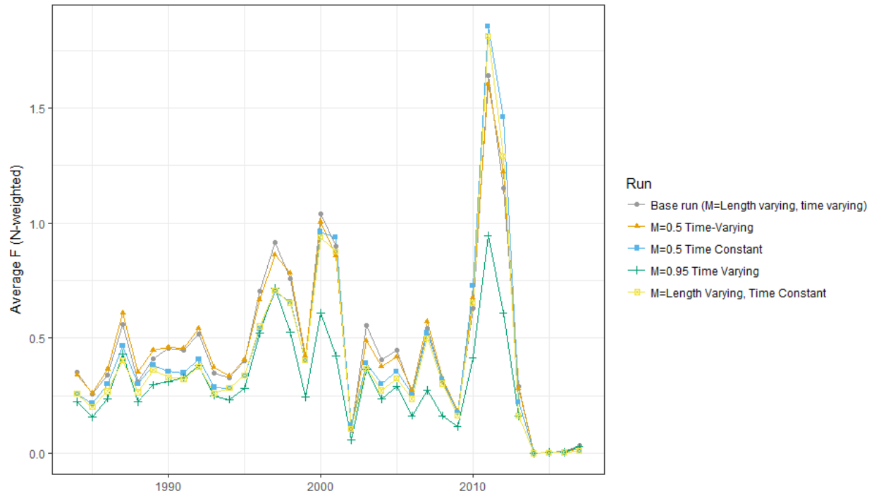
Figure 5.32. Average F estimates from the UME model under different M scenarios.
