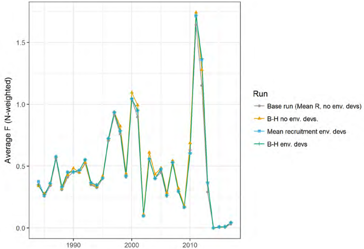
Figure 5.40. Estimates of average F from the UME model fit with and without an environmental index of recruitment deviations.
