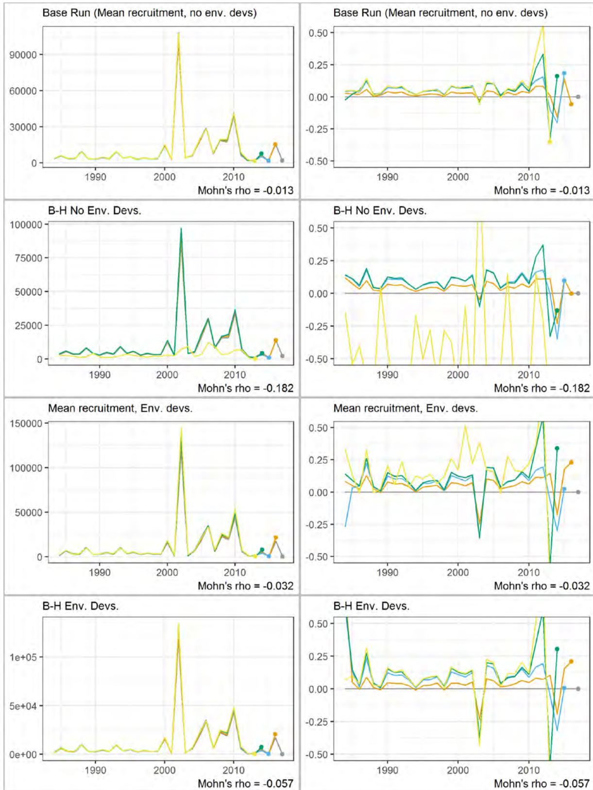
Figure 5.41. Recruitment retrospective patterns from the UME model fit with and without an environmental index of recruitment deviations.
