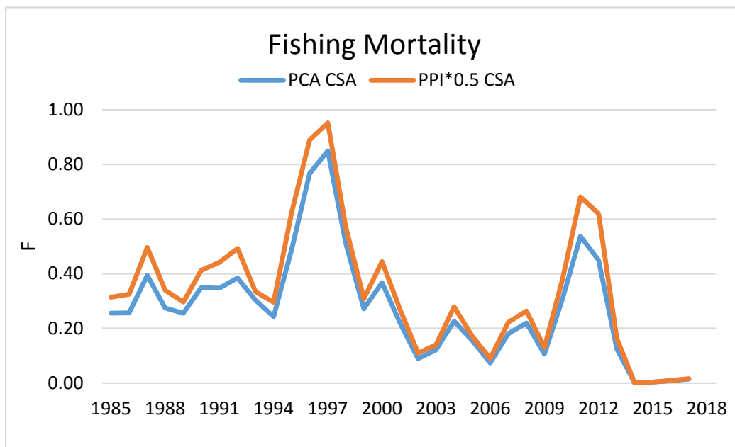
Figure 5.7. (a-d) Comparison of CSA estimates from final model ( M=0.5 \cdot PPI ) and PCA model where M was scaled using a composite environmental variable incorporating both temperature and predation. (a) recruit abundance, (b) post recruit abundance, (c) exploitable biomass, (d) F .
