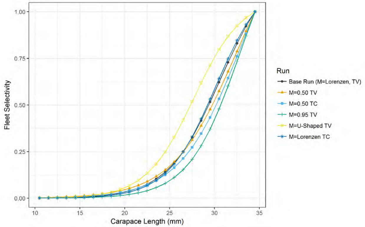
Figure A32. Mixed fleet selectivity patterns for the new base run of the UME model under different M scenarios.
