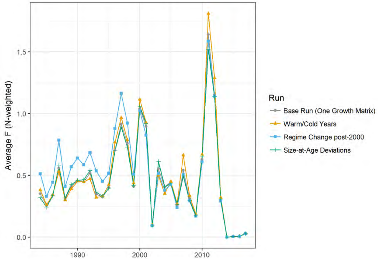
Figure 5.51. Estimates of average F from the UME model under different growth block scenarios.
