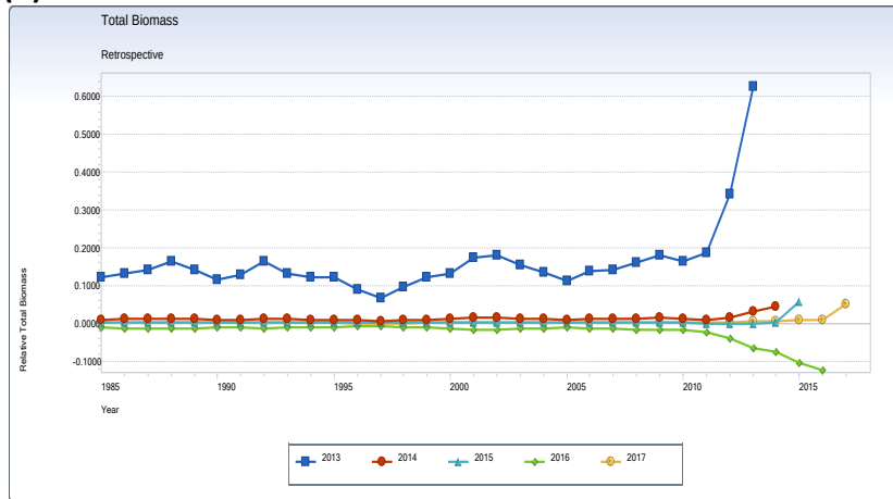
Figure 5.3 (a-h) Retrospective patterns for CSA final run using M=0.5 \times \text{PPI} and model-based indices. (a) F retrospective, (b) F relative retrospective, (c) recruits retrospective, (d) recruits relative retrospective, (e) post recruits retrospective, (f) post recruits relative retrospective, (g) total biomass retrospective, (h) total biomass relative retrospective.
