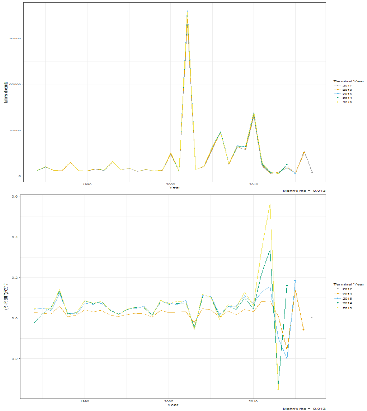
Figure 5.22. Retrospective analysis results for recruitment for the base run of the UME model. Absolute values top, relative to 2017 run bottom.
