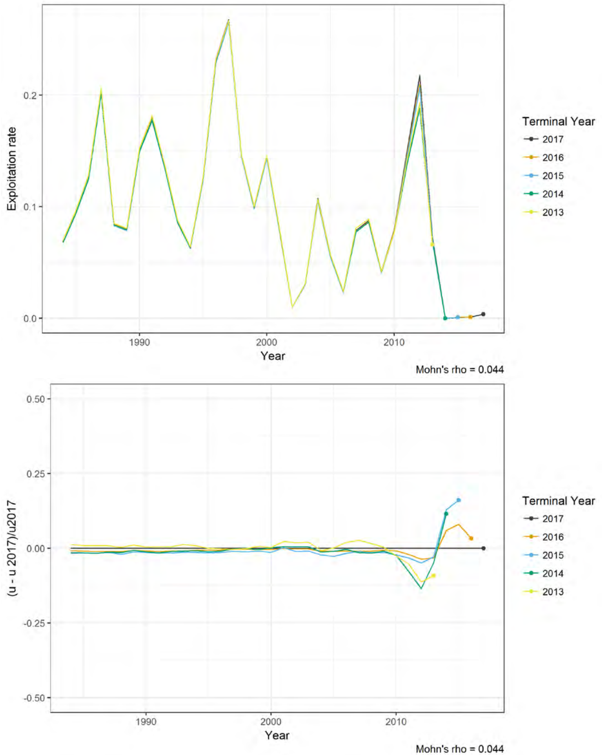
Figure A14. Retrospective pattern for exploitation rate on the absolute (top) and relative (bottom) scale.
