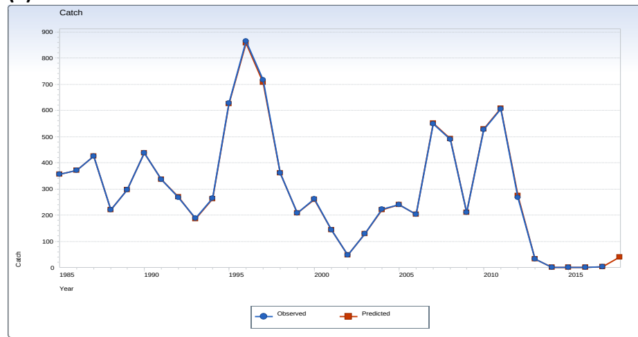
Figure 5.1 (a-e) CSA model fits to survey indices and catch using model-based indices and PPI-scaled M (based on M=0.5 ). (a) pre-recruits, (b) post-recruits, (c) fall albatross survey data, (d) fall Bigelow survey data (e) catch.
