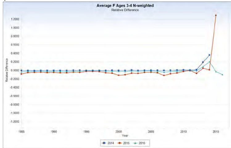
Figure 5.62 (a-r) Retrospective patterns for ASAP final run using model-based indices and age-varying and time varying (PPI scaled) M (based on M=0.5 ). (a) SSB; (b) relative change in estimates of SSB; (c) January 1 biomass; (d) relative change in estimates of January 1 biomass; (e) exploitable biomass; (f) relative change in estimates of exploitable biomass; (g) total stock numbers; (h) relative change in estimates of total stock numbers; (i) age 1 stock numbers; (j) relative change in estimates of age 1 stock numbers; (k) age 2 stock numbers; (l) relative change in estimates of age 2 stock numbers; (m) age 3 stock numbers; (n) relative change in estimates of age 3 stock numbers; (o) age 4 stock numbers; (p) relative change in estimates of age 4 stock numbers; (q) average F for ages 3-4; (r) relative change in estimates of average F for ages 3-4.
