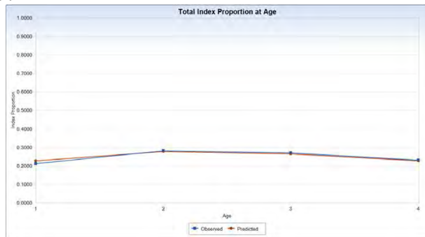
Figure 5.60 (a-c) ASAP model fits to proportion at age for survey indices a) Summer Survey, b) NEFSC Albatross, c) Bigelow, for time- and age-varying M (based on M=0.5 ).
