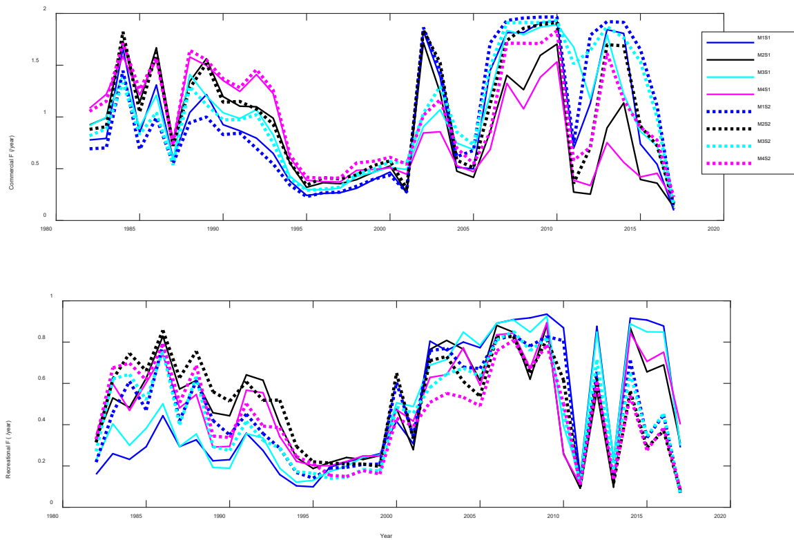
Figure 36. Sensitivity results for commercial (top) and recreational (bottom) fishing mortality estimated by Bayesian age- structured models using the new (S1, solid lines) and old (S2, dashed lines) MRIP estimates, plotted together. M4 is the preferred model.
