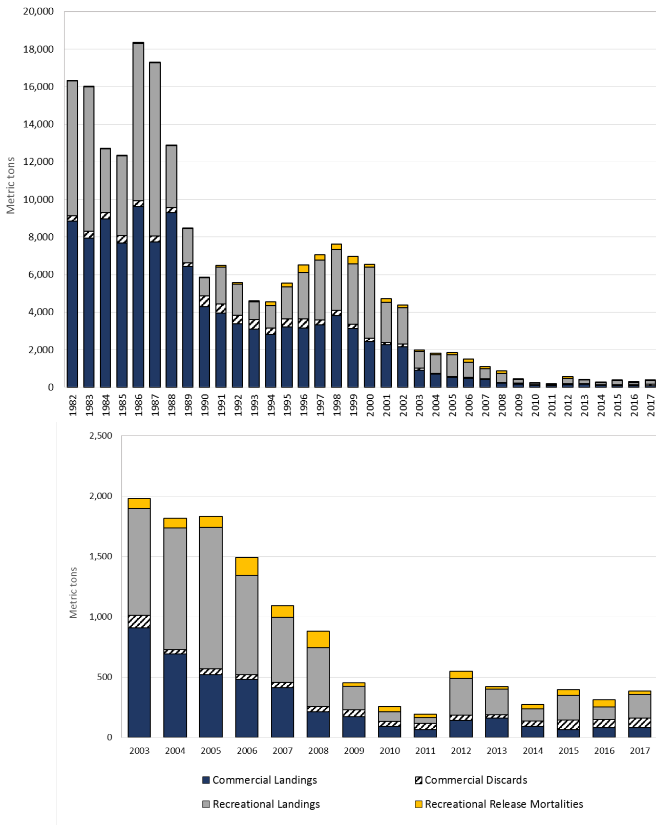
Figure 4. Total annual weakfish removals by sector used in the assessment. Top figure is 1982-2017, bottom figure is 2003 – 2017 to show detail in recent years.
