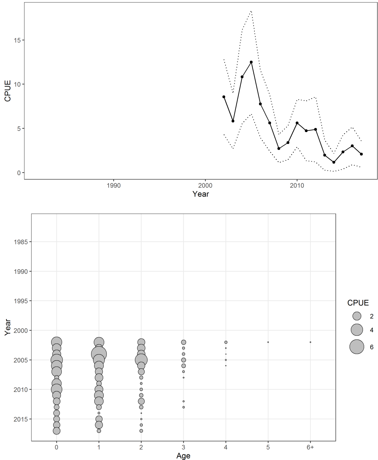
Figure 12. ChesMMA age-1+ index with 95% confidence intervals (top) and ChesMMA index-at-age (bottom).
