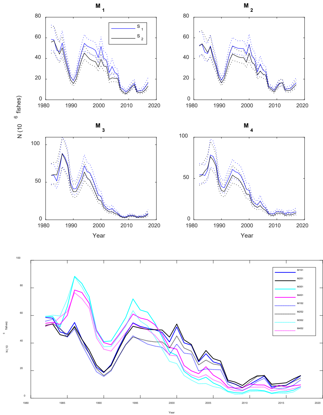
Figure 38. Sensitivity results for weakfish total abundance estimated by Bayesian age- structured models using the new (S1) and old (S2) MRIP estimates. M4 is the preferred model. Solid line = posterior mean; dashed lines = 95% credible interval.
