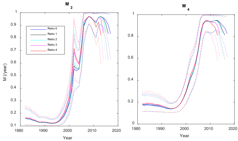
Figure 43. Retrospective analysis results of M estimates from the nonstationary Bayesian statistical catch-at-age models. M_4 is the preferred model. Solid line = posterior mean; dashed lines = 95% credible interval.
