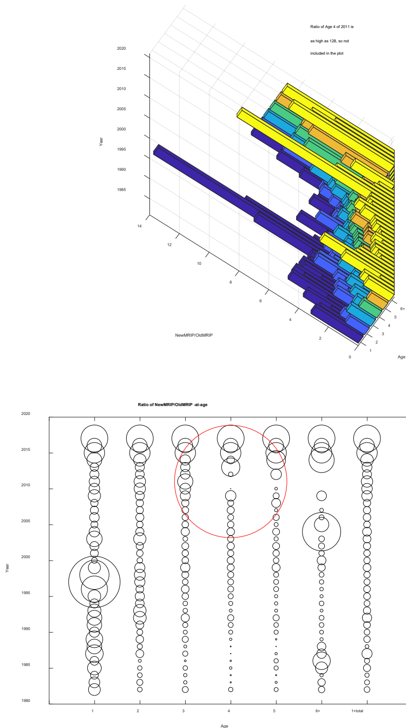
Figure 34. Differences in the changes of the newly estimated MRIP (New MRIP/Old MRIP) among ages and year shown as 3D bar plot (top) and bubble plot (bottom). The red circle in the bottom plot is the ratio of age 4 of 2011 recreational catch.
