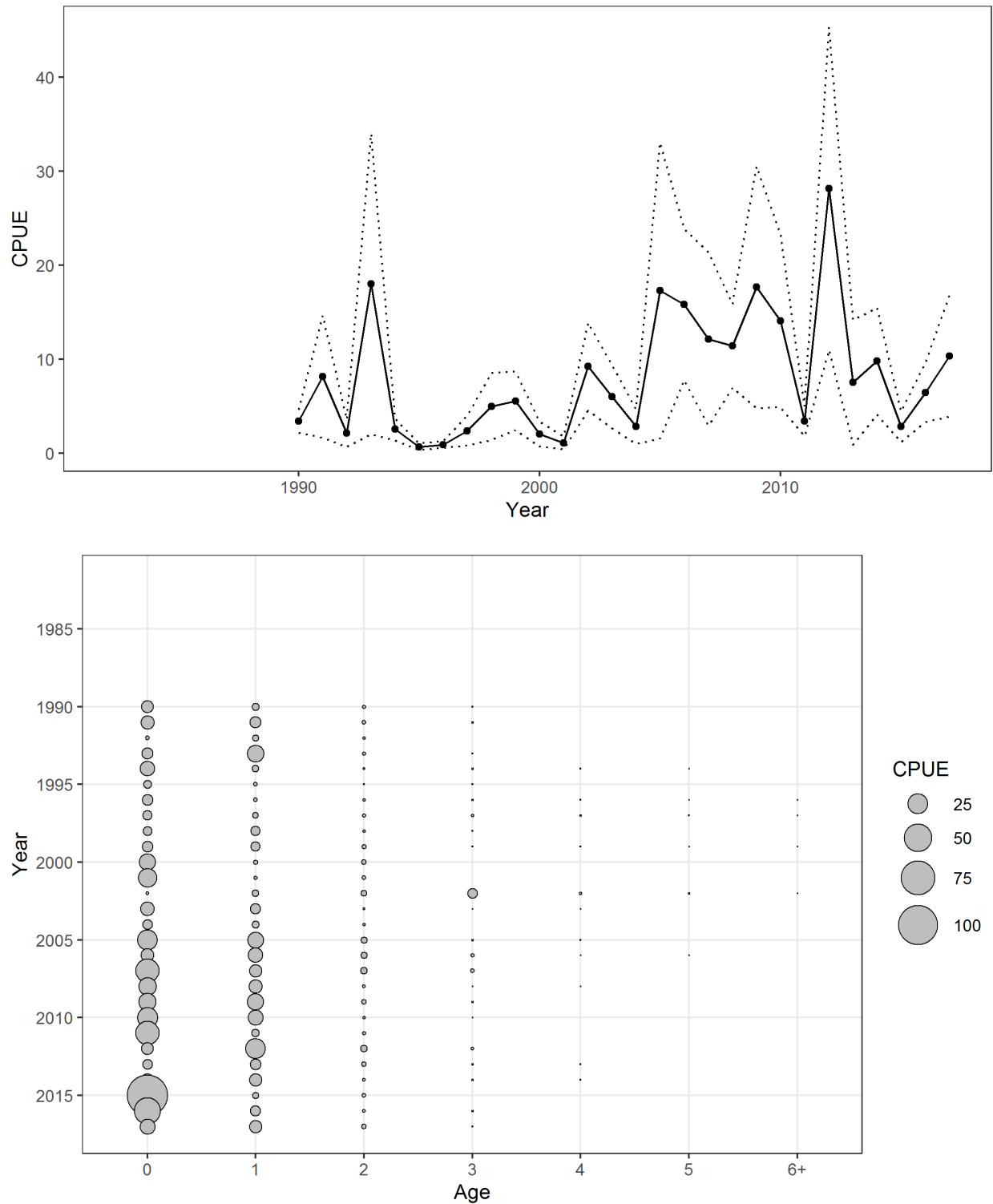
Figure 8. SEAMAP age-1+ index with 95% confidence intervals (top) and SEAMAP index-at-age (bottom).
