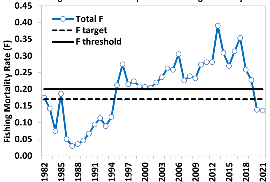
Figure 3. Atlantic Striped Bass Fishing Mortality
