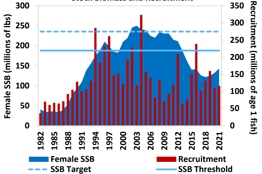
Figure 2. Atlantic Striped Bass Female Spawning Stock Biomass and Recruitment
