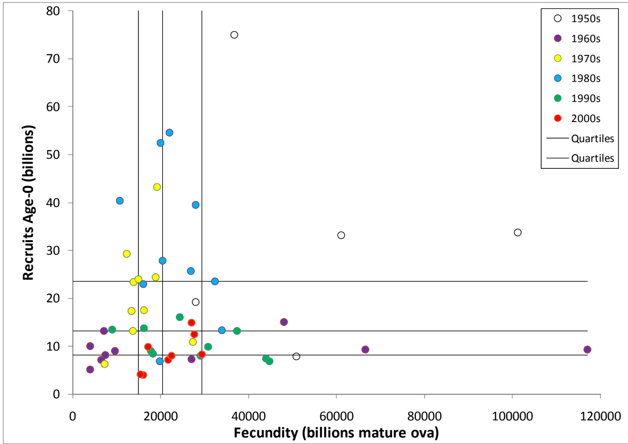
Figure 8.3 Plot of Atlantic menhaden fecundity (billions of mature ova) and age-0 recruitment (billions) estimates lagged by one year from the base BAM model.
