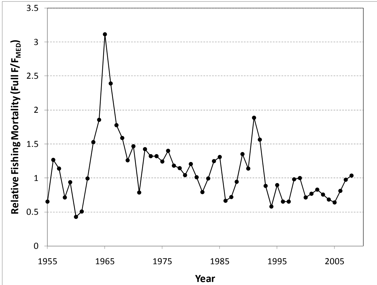
Figure 8.4. Annual fishing mortality rate (full F) relative to F_{MED} = 2.20 for base run (for comparison: F_{target} = 0.96 ).
