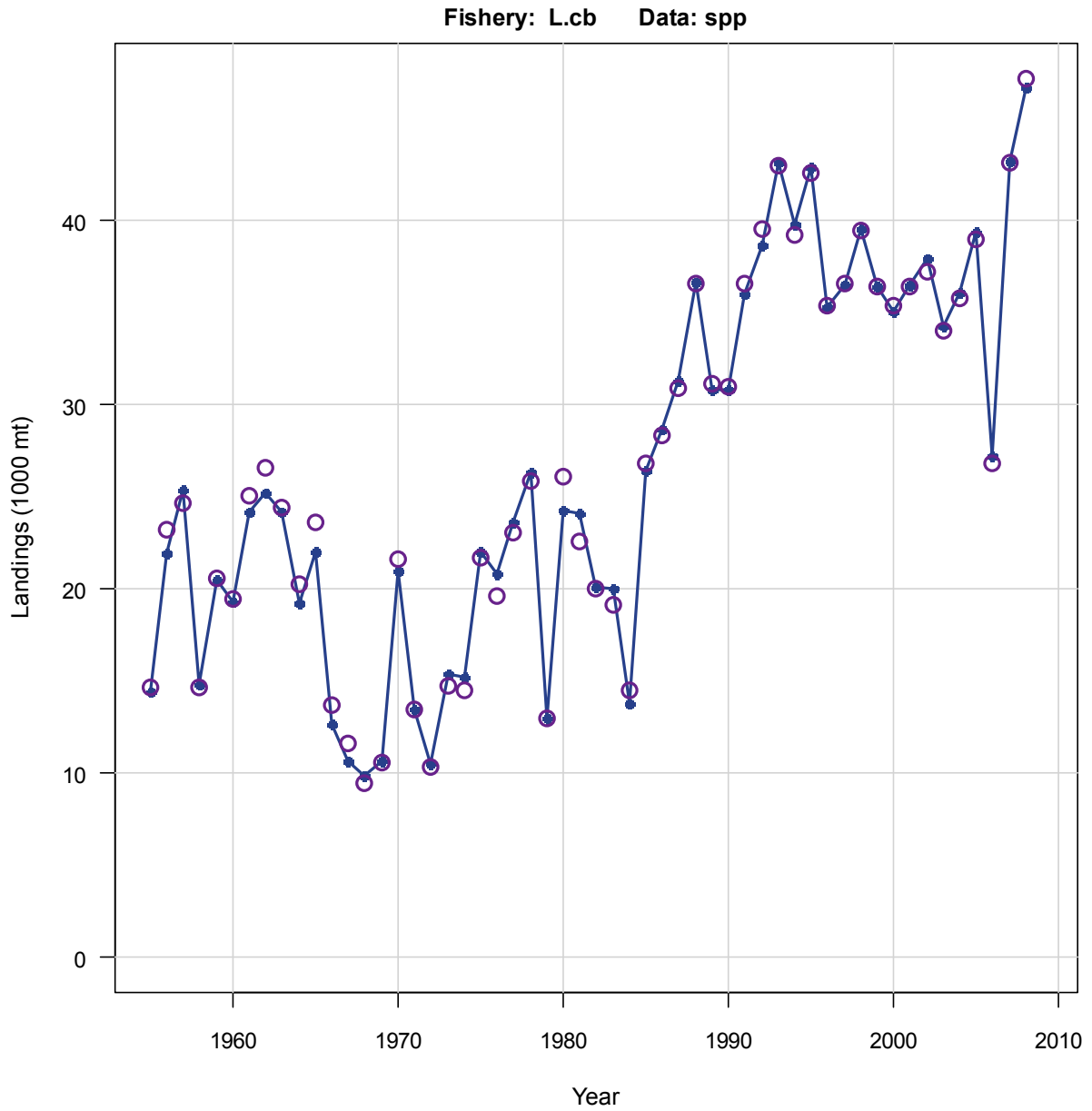
Figure 7.2 Observed (open circles) and predicted (connected points) landings in 1000 metric tons of Atlantic menhaden by the bait fishery from the base BAM model.
