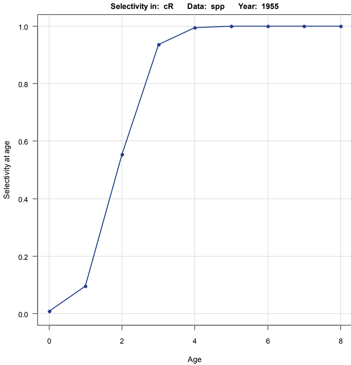
Figure 7.9 Estimated age-specific selectivity pattern for the Atlantic menhaden commercial reduction fishery from the base BAM model.
