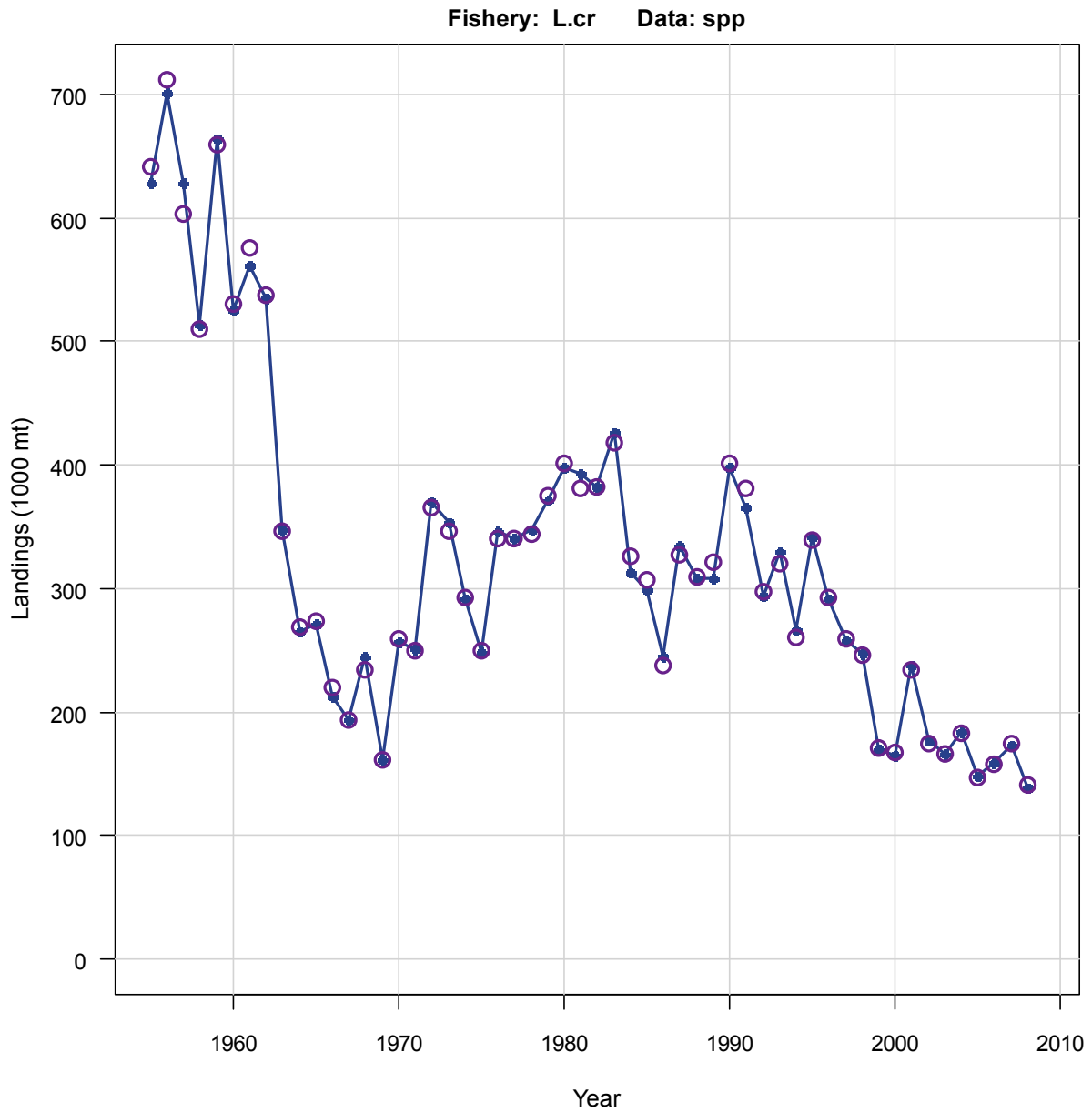
Figure 7.1 Observed (open circles) and predicted (connected points) landings in 1000 metric tons of Atlantic menhaden by the commercial reduction fishery from the base BAM model.
