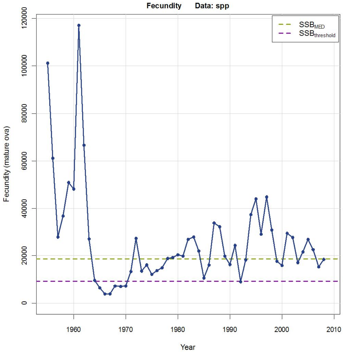
Figure 8.5. Annual fecundity compared to target and limit.
