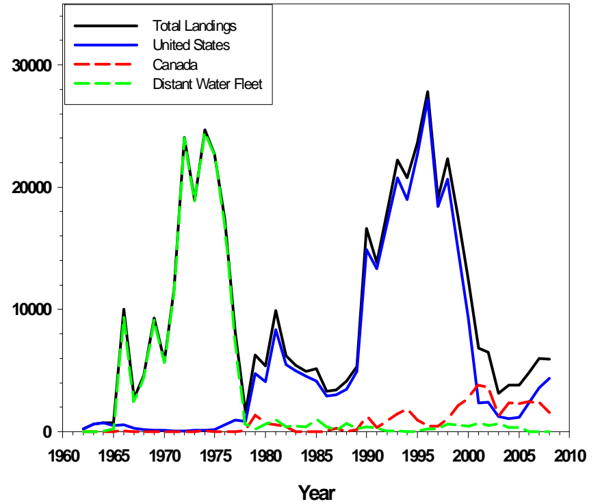
Figure 2. Total landings of spiny dogfish from US, Canada, and the distant-water fleet.
