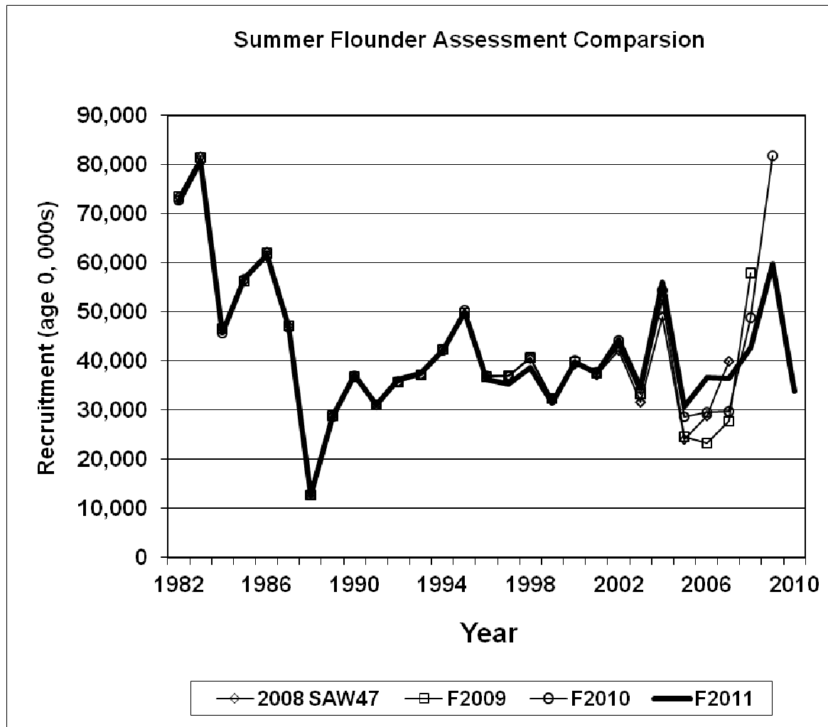
Figure 24. Comparison of the estimates for Recruitment from the 2008 SAW47 and 2009-2011 updated assessments.
