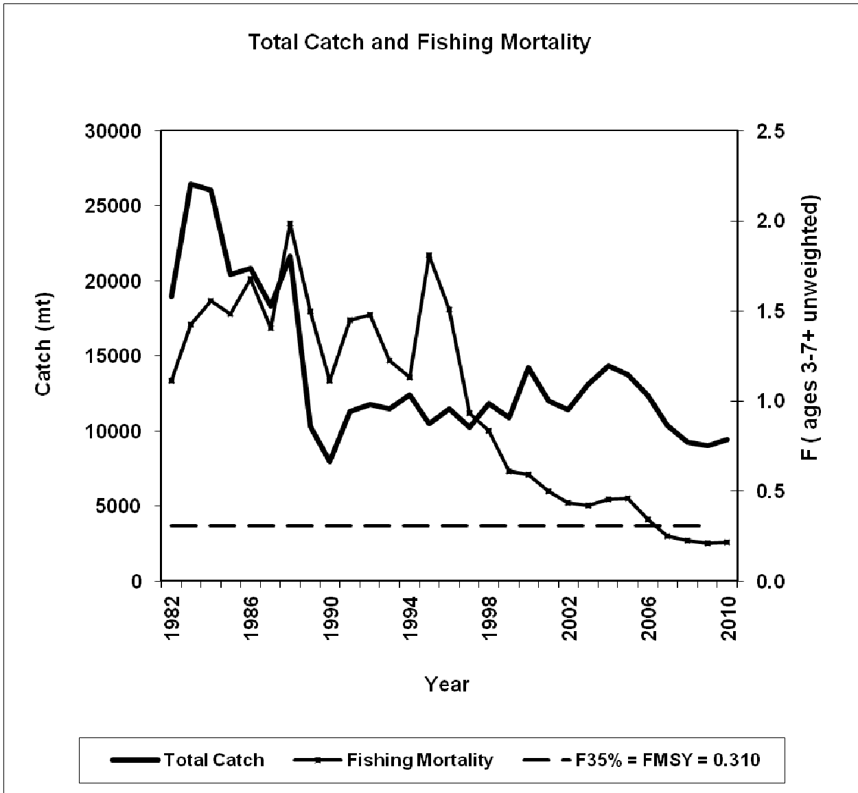
Figure 15. Total fishery catch and fishing mortality rate (F, ages 3-7+) for summer flounder. F35% is the proxy for FMSY.
