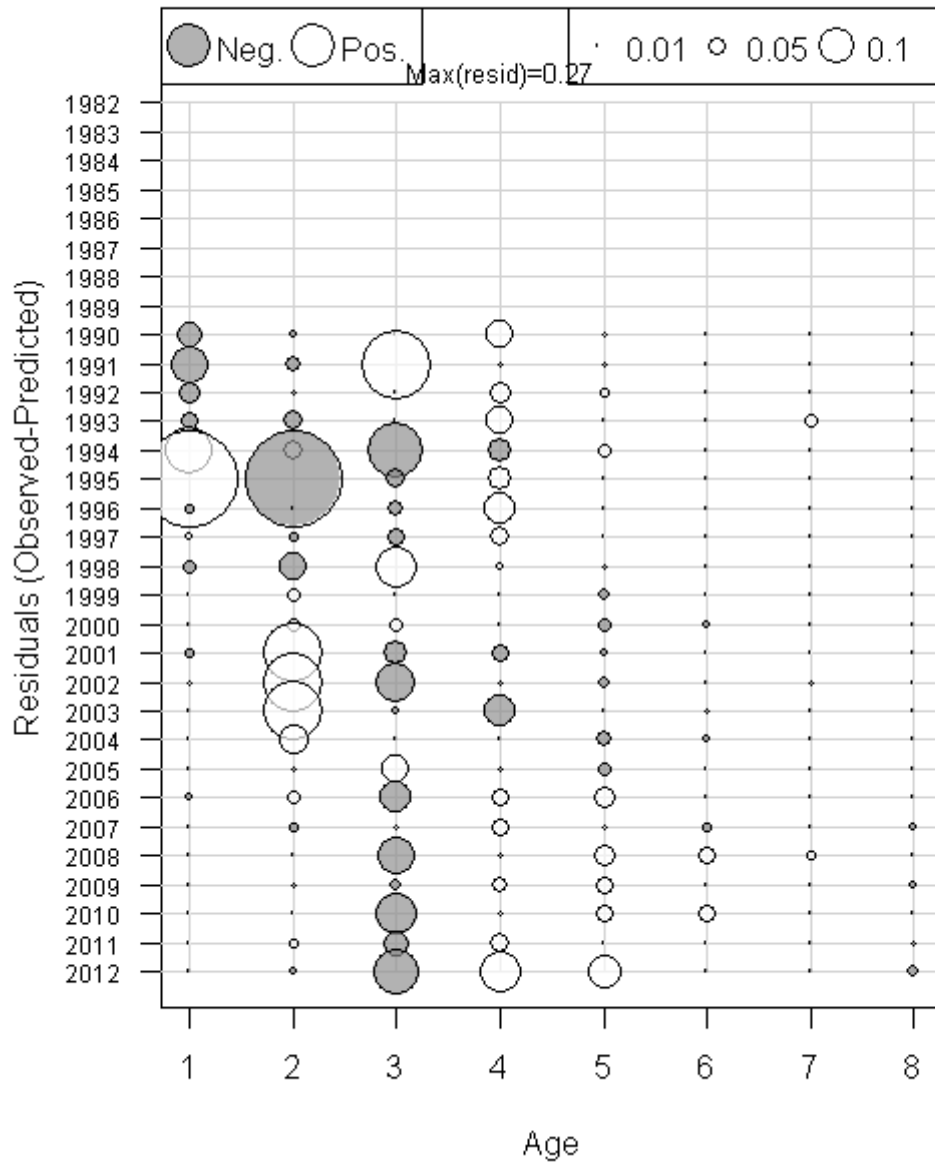
Figure A213. Age composition residuals for the RIDFW monthly fixed station trawl survey in run F57_BASE_12.
