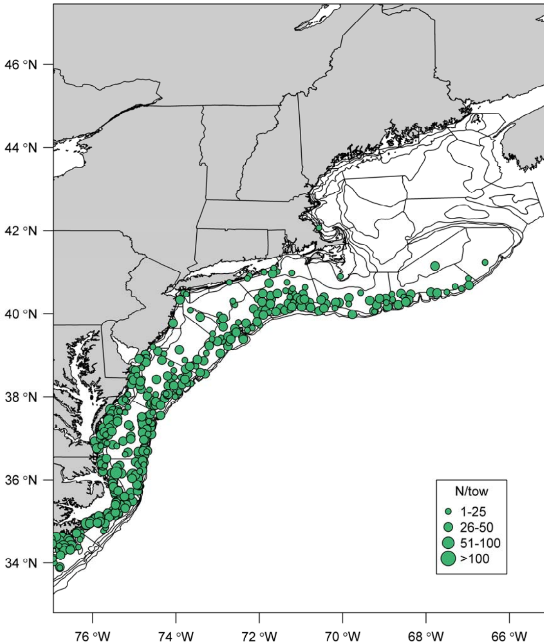
Figure A98. NEFSC spring survey catch numbers per tow, 1981-1985.
