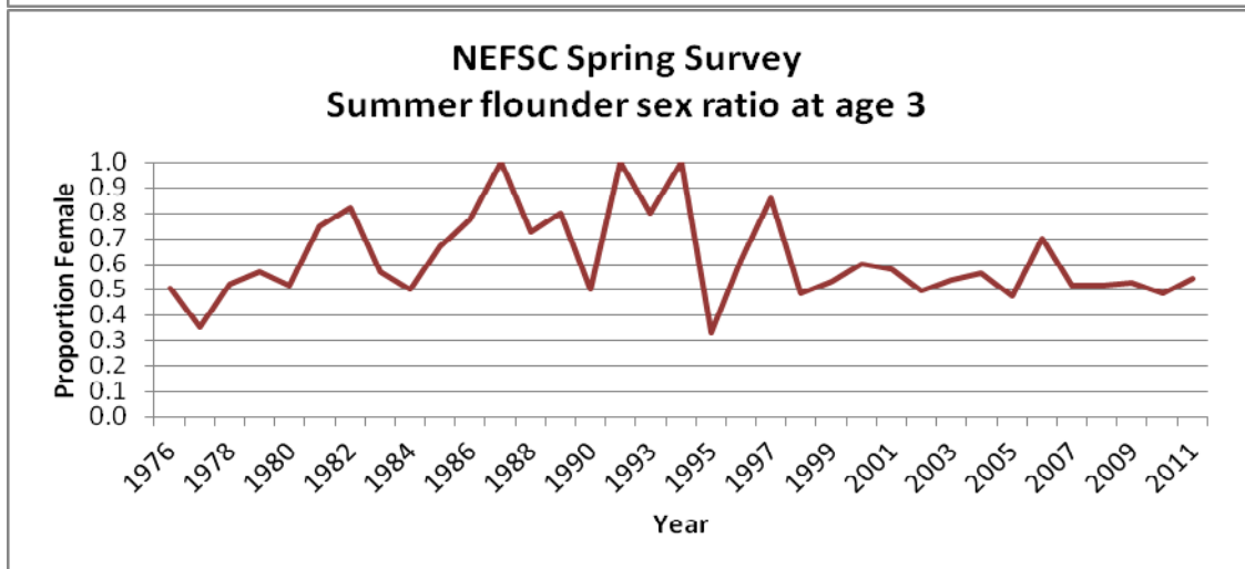
Figure A162: NEFSC spring survey: proportion female at ages 1-3.
