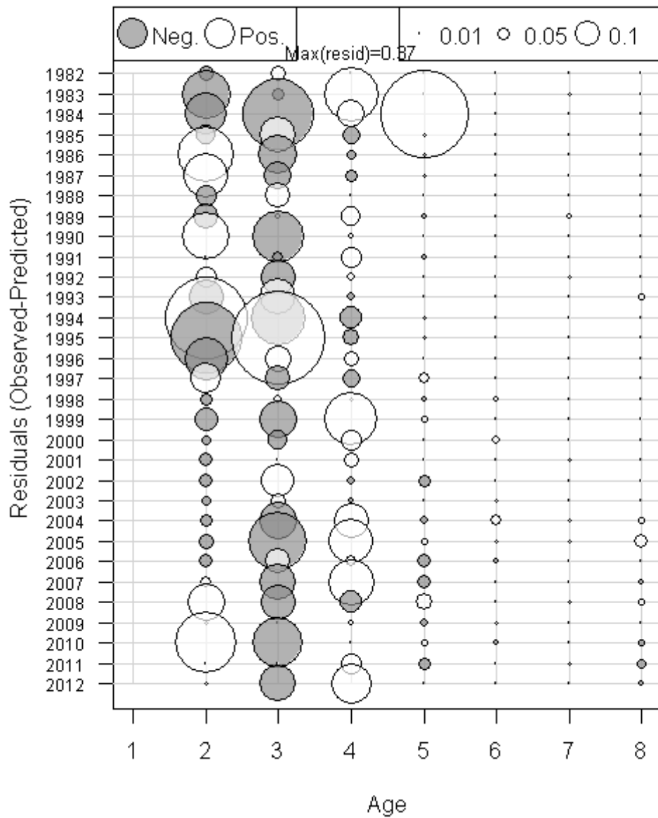
Figure A207. Age composition residuals for the MADMF spring trawl survey in run F57_BASE_12.
