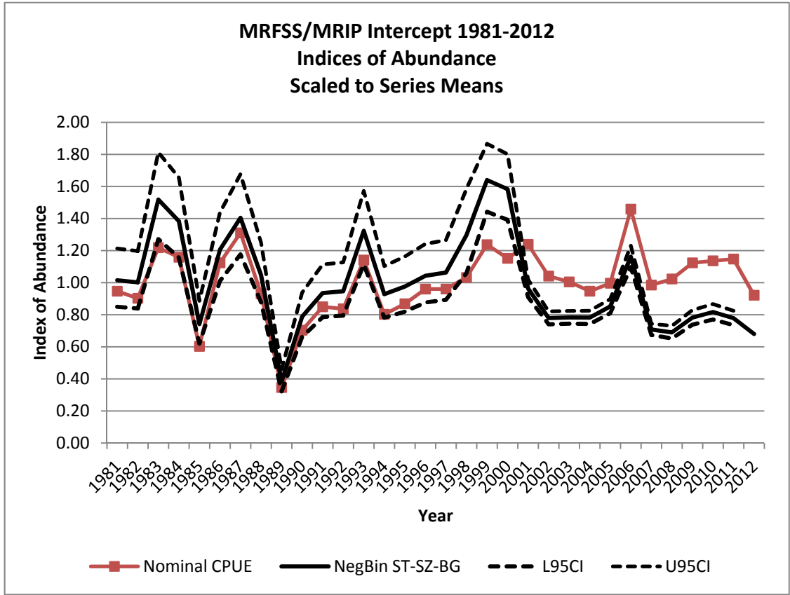
Figure A156. Comparison of the MRFSS/MRIP intercept negbin six-factor ST-SZ-BG model-based indices and the nominal index.
