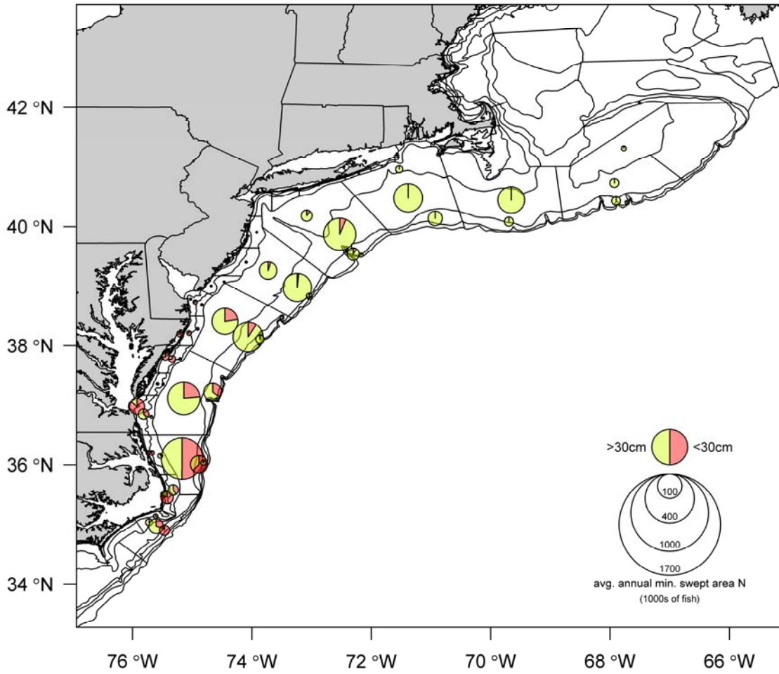
Figure A110. NEFSC spring survey average minimum swept area abundances by strata and size category, 1996-2000.
