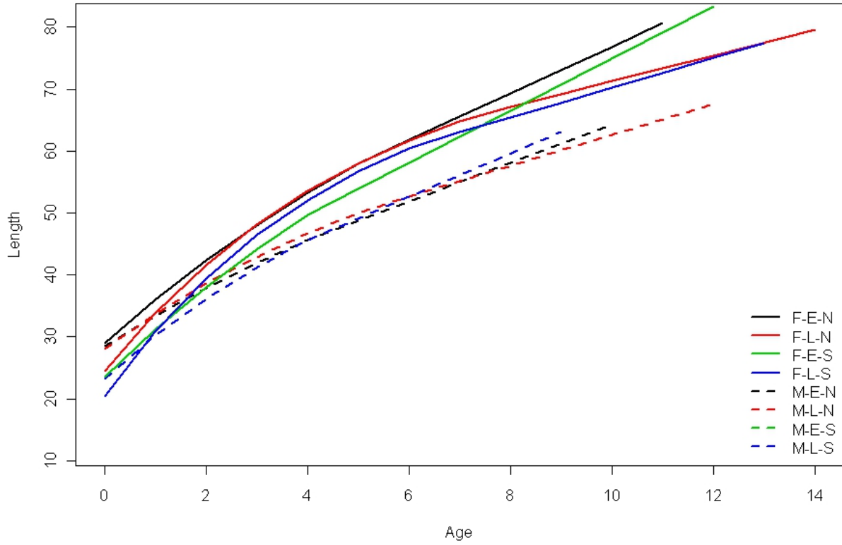
Figure A177. All model fits by strata shown together for comparison.
