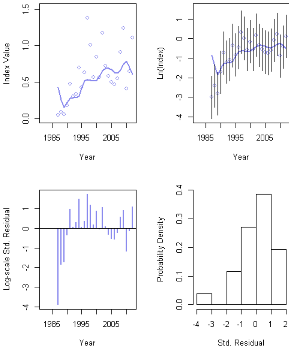
Figure A233. Fit diagnostics for the NYDEC trawl survey in run F57_BASE_12.
