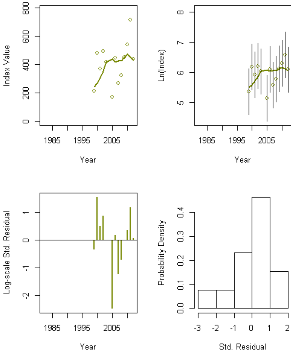
Figure A237. Fit diagnostics for the NEFSC ECOMON larval survey in run F57_BASE_12.
