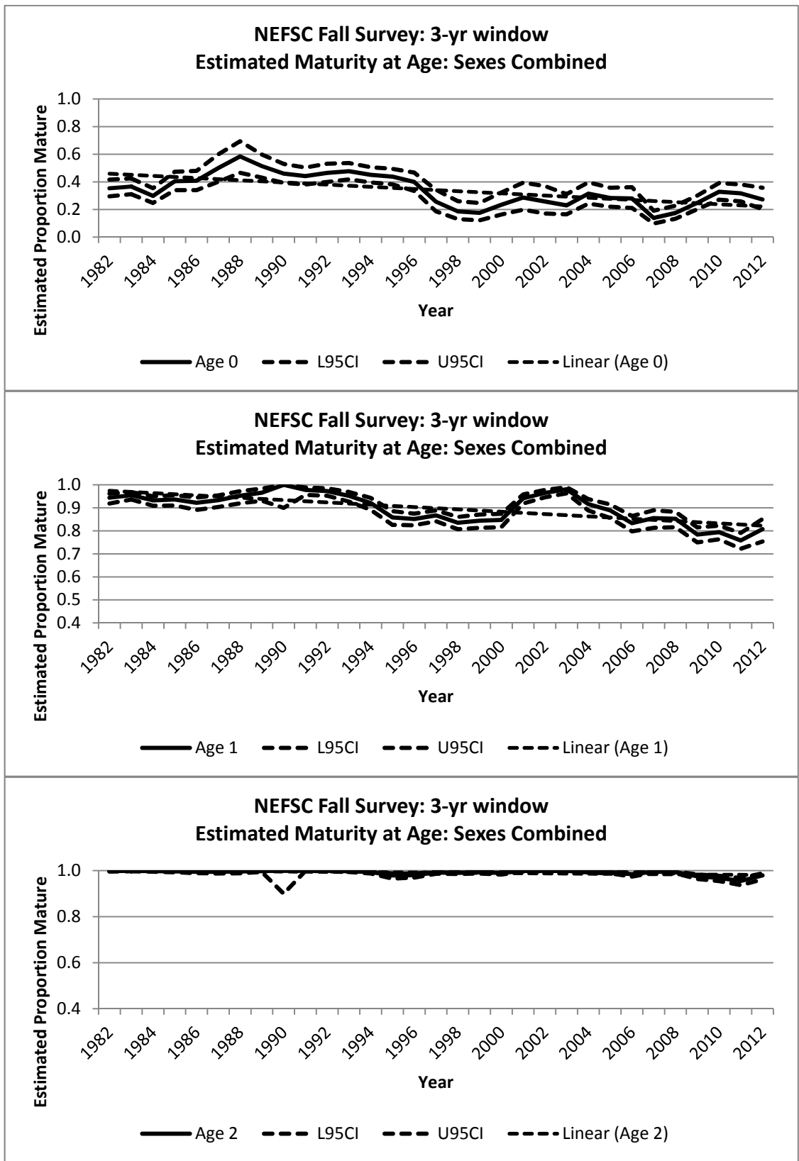
Figure A35. Estimated maturity at ages, 0, 1, and 2, for sexes combined by 3-year moving window. Straight dashed lines are fit linear trends.
