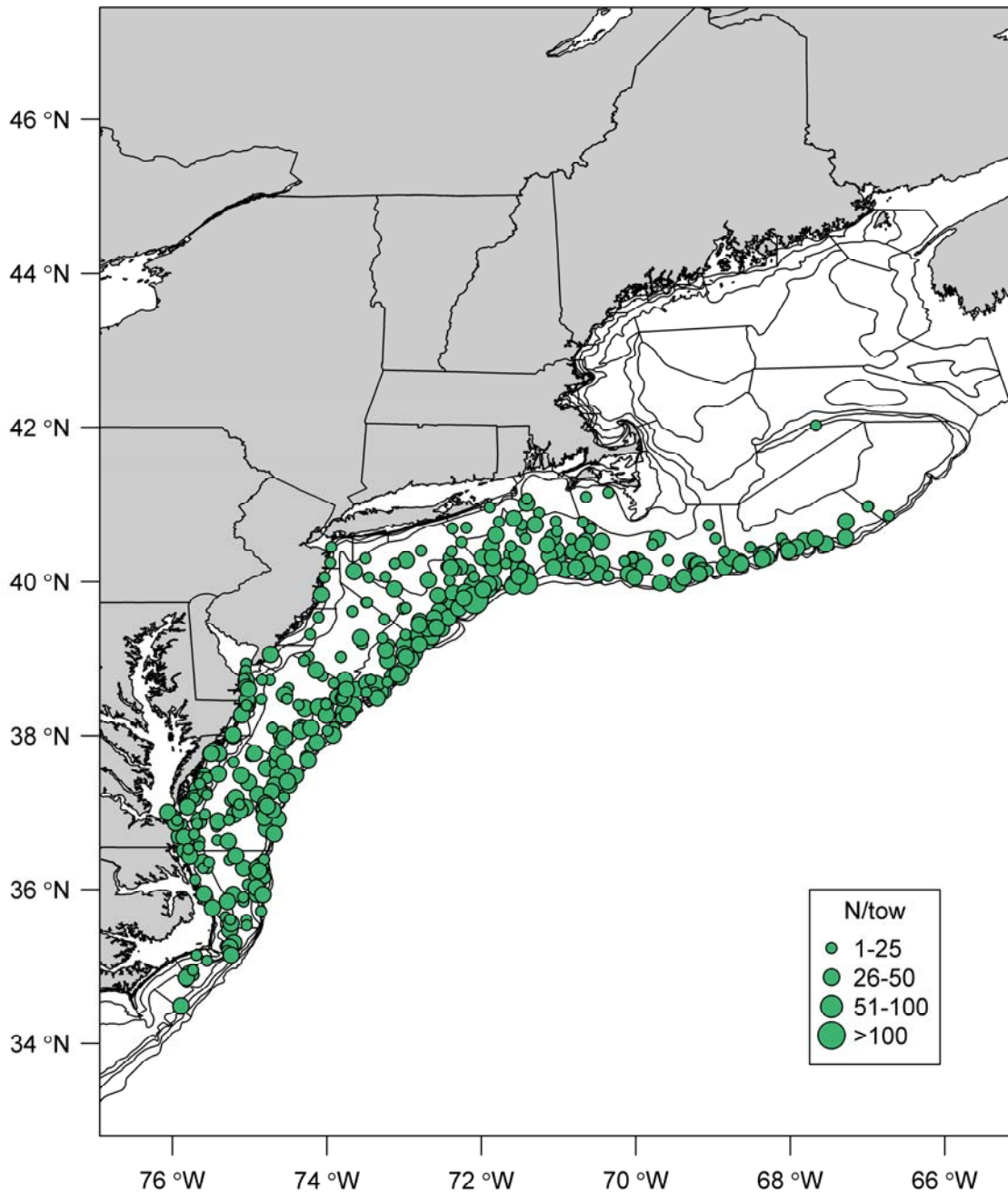
Figure A102. NEFSC spring survey catch numbers per tow, 2001-2005.
