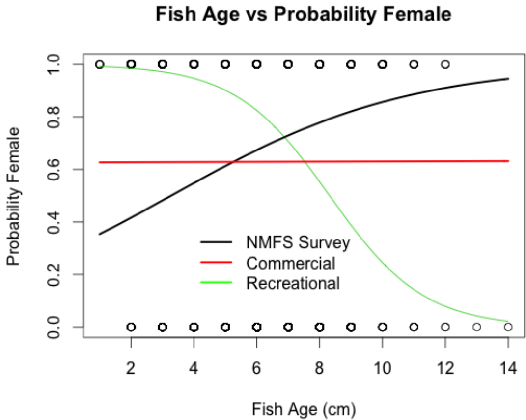
Figure A182. Probability female as a function of fish age in the commercial and recreational fisheries (2010-2011) and the NMFS-NEFSC trawl survey (2009-2011) with separate logistic regression parameters estimated for each line.
