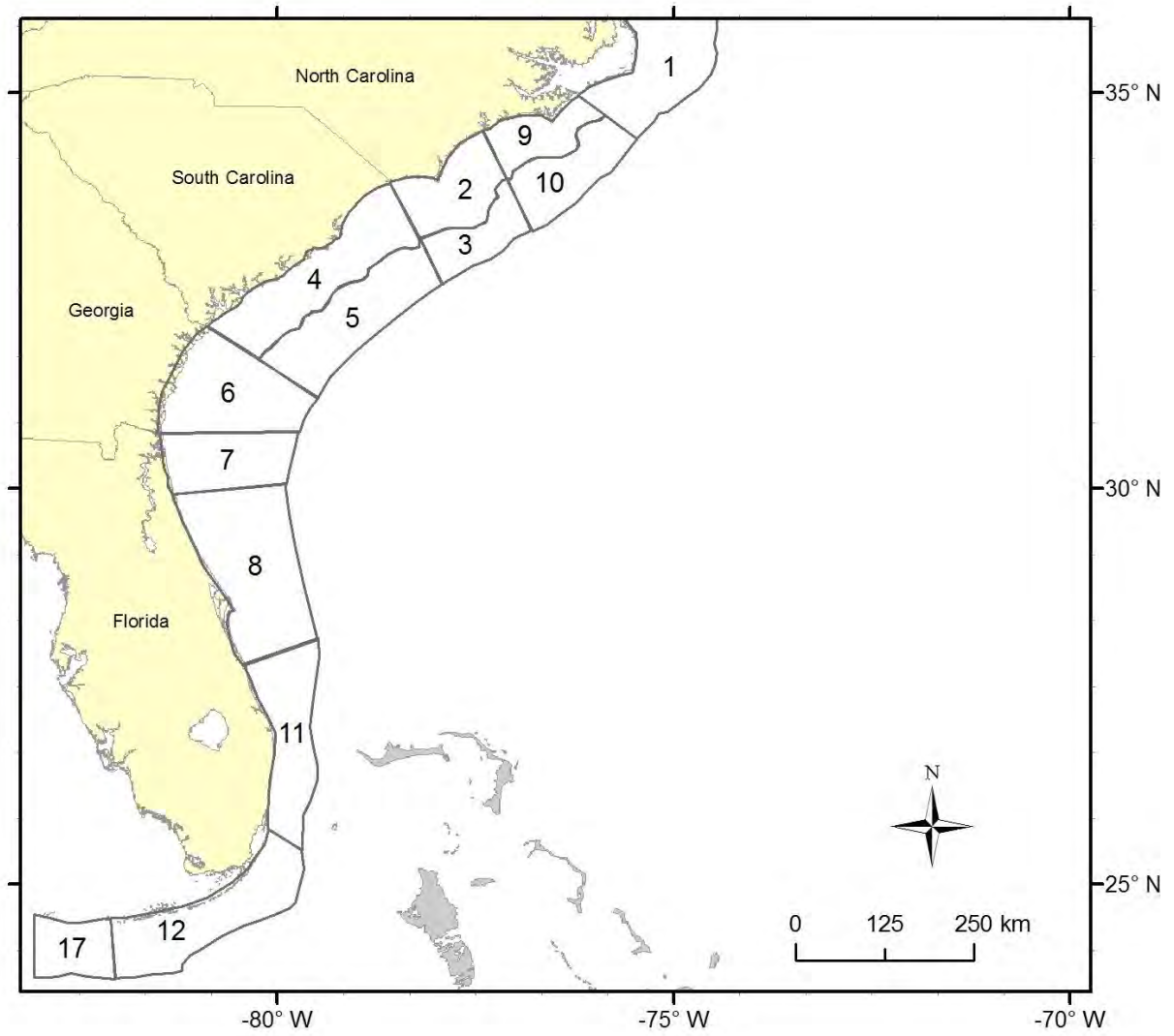
Figure 5.4.1.1. Map of headboat sampling area definition. These areas were pooled into regions of North Carolina (NC=1,2,3,9,10), South Carolina (SC=4,5), and Georgia (GA=6).
