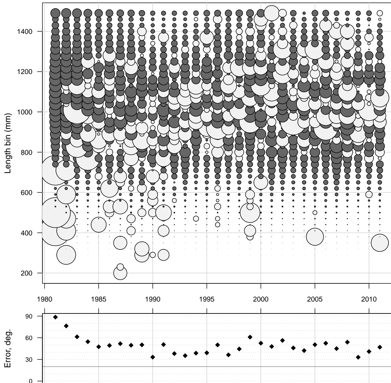
Figure 3.3. Top panel is a bubble plot of length composition residuals from the general recreational fishery. Dark represents overestimates and light indicates underestimates. Bottom panel shows the angle (in degrees) between vectors of observations and estimates, with a reference line at 20 degrees. Error is bounded between 0 and 90 degrees, with 0 indicating a perfect fit.
