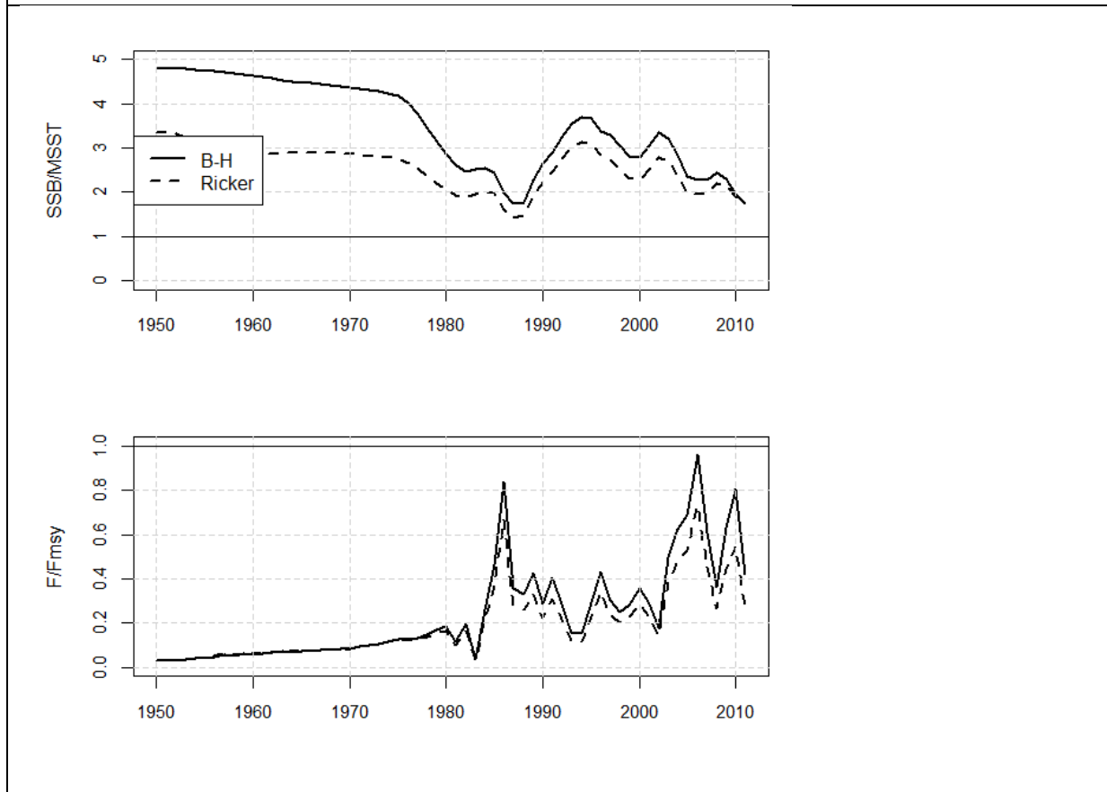
Comparison of stock status and exploitation status with alternative BH or Ricker S-R relationships.
