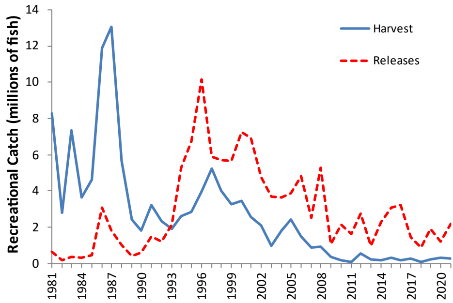
Figure 4. Recreational weakfish harvest and releases (number of fish), from 1981 to 2021 (see Tables 5 and 6 for source information and values).
