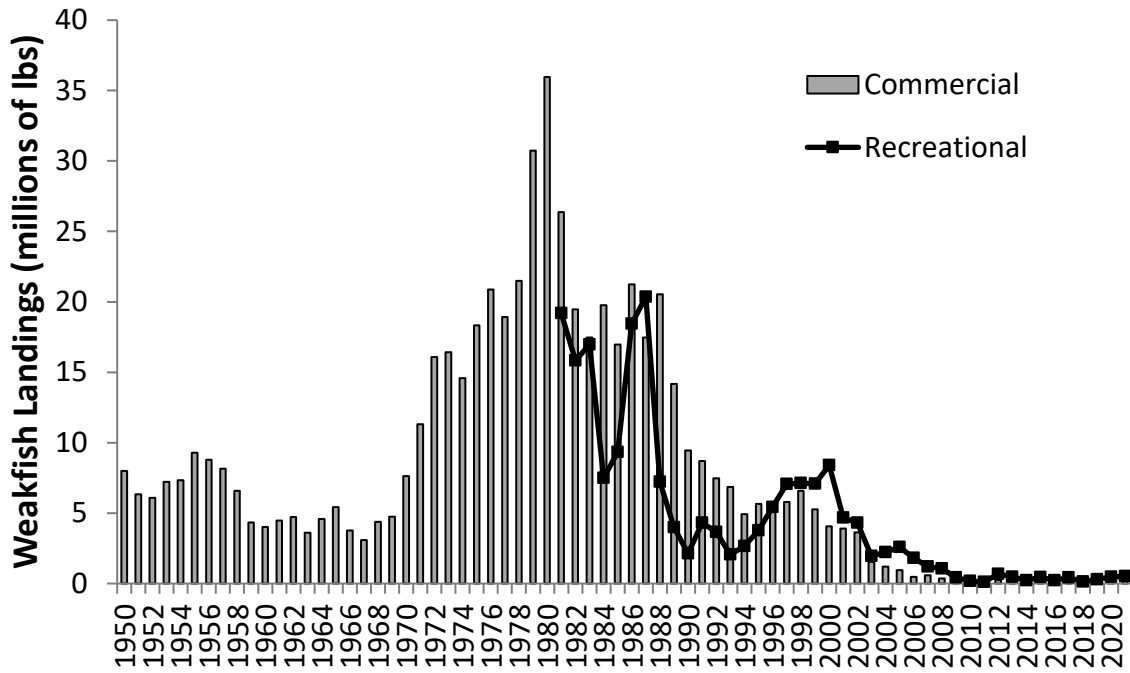
Figure 2. Commercial and recreational weakfish harvest (pounds), from 1950 to 2021 (see Tables 3 and 4 for source information and values). Recreational data is unavailable prior to 1981.
