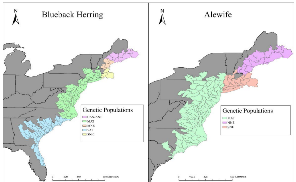
Figure 1. Genetic stock-regions of river herring. Five genetic populations for blueback herring (Canada-Northern New England, Mid-New England, Southern New England, Mid-Atlantic, and South Atlantic) and three genetic populations for alewife (Northern New England, Southern New England [SNE], and Mid- Atlantic).
